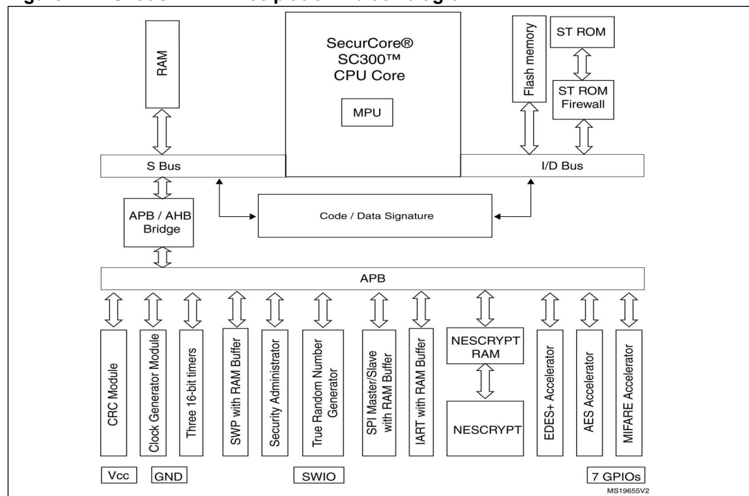
Figure 1. ST33G1M2A1 C05 platform block diagram
