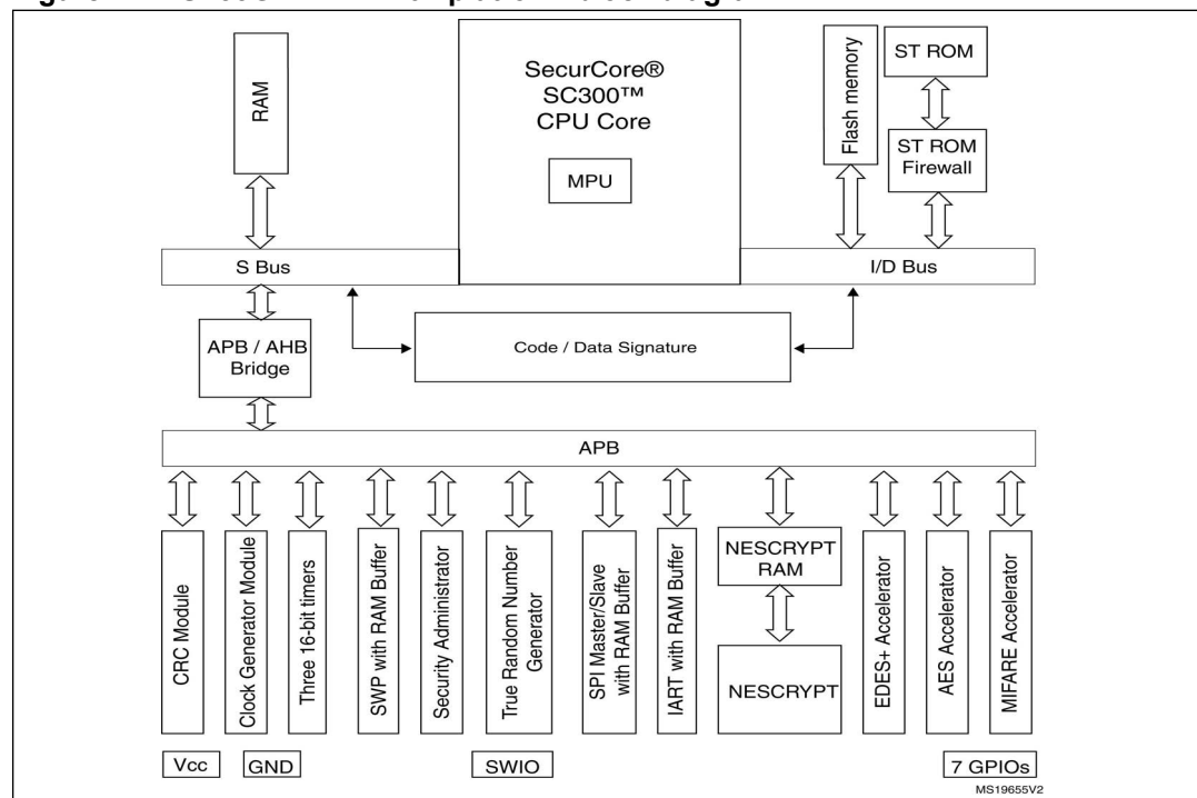
Figure 1. ST33G1M2AM C04 platform block diagram
