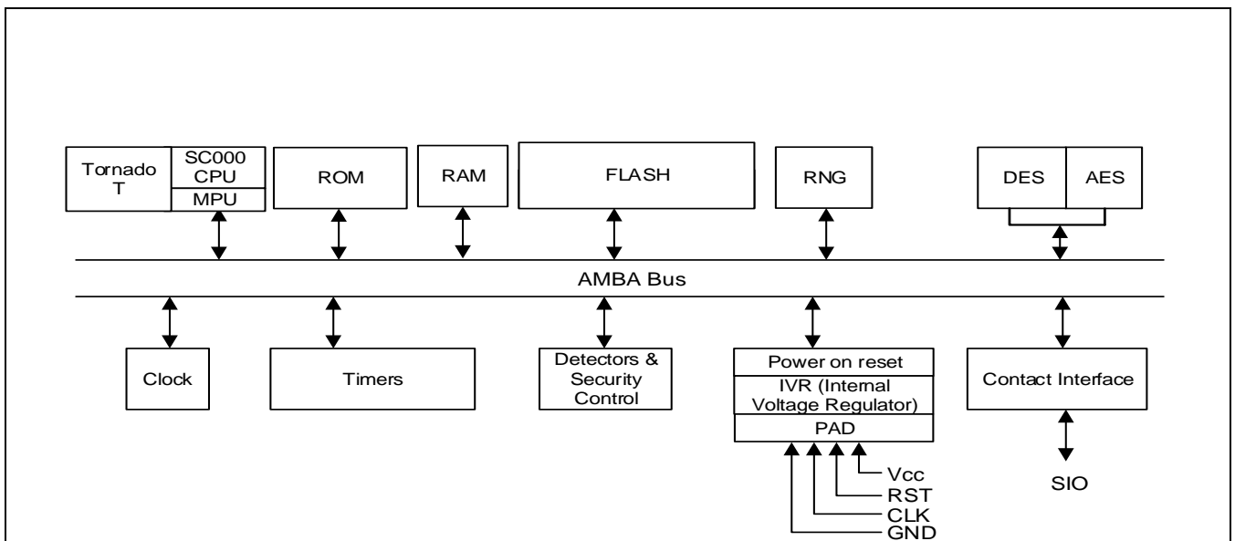
Figure 1 S3K250A/S3K232A/S3K212A Block Diagram
