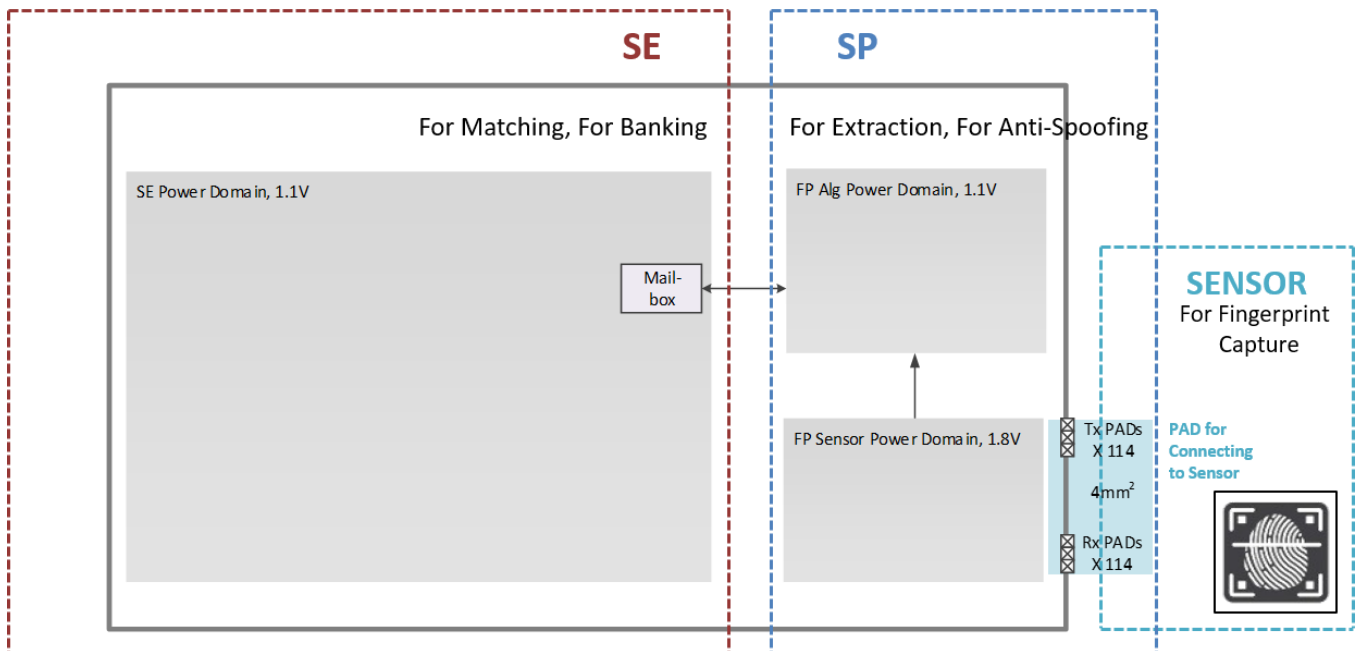
Figure 1-2 S3B512C/SC3512C Architecture
