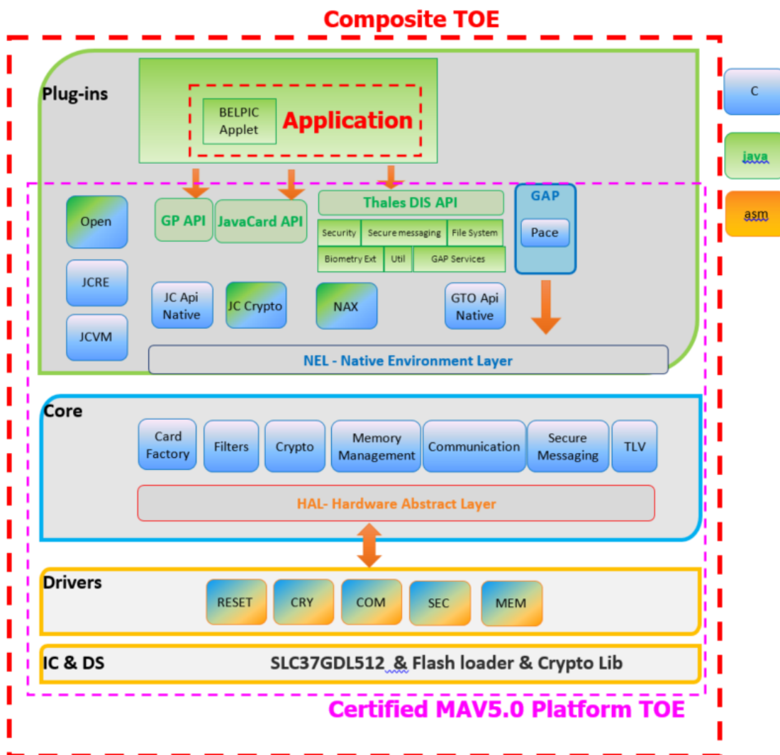
Figure 1: BELPIC TOE boundaries
