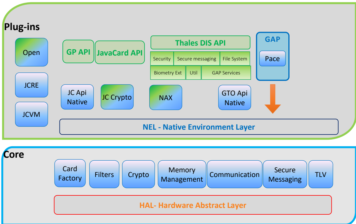
Figure 2: MultiApp V5.0 Javacard Platform Architecture
