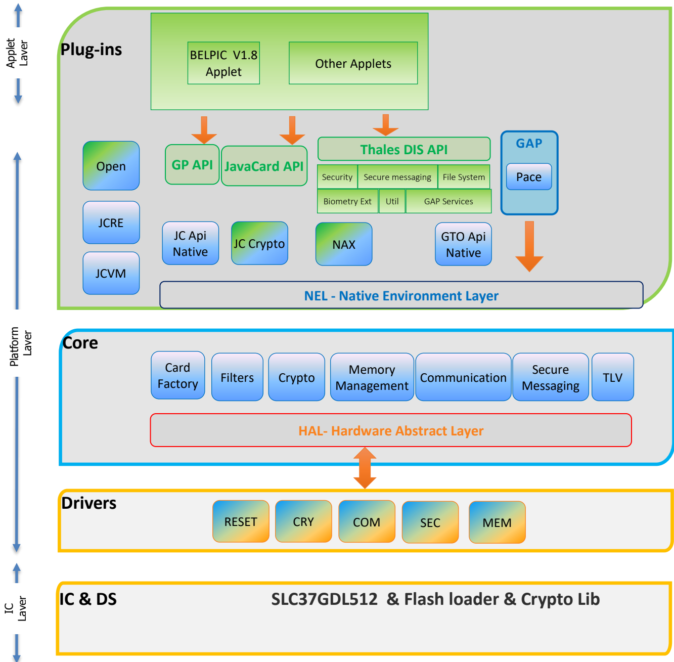
Figure 3: BELPIC Electronic Identity Card structure
