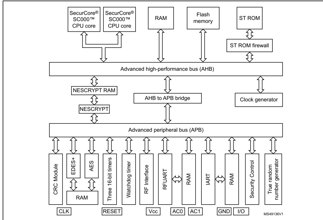
Figure 1. ST31P450 B05 platform block diagram
