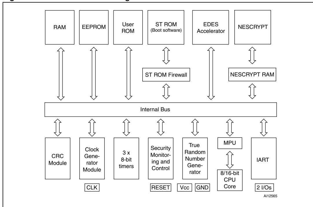
Figure 1. SA23YL18A block diagram
