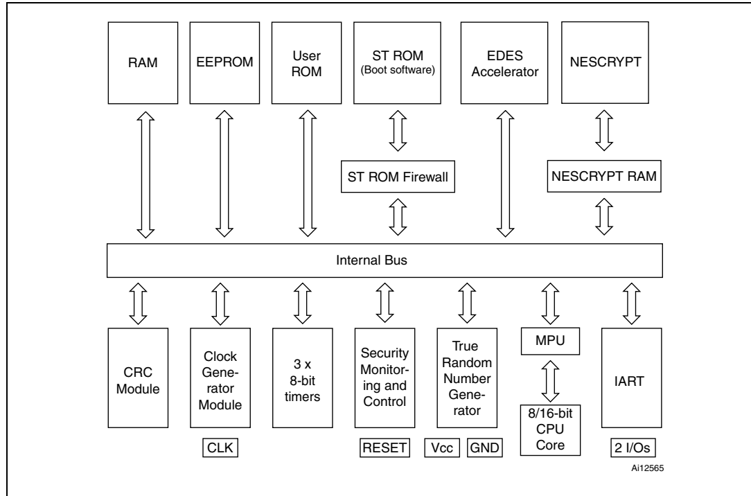
Figure 1. ST23YL18A block diagram
