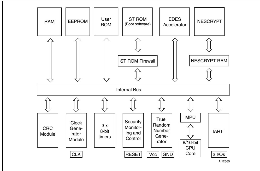
Figure 1. ST23YL18B block diagram
