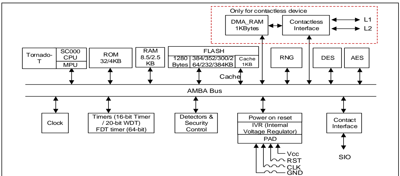
Figure 1 S3D384C/S3D352C/S3D300C/S3D264C/S3D232C/S3K384C Block Diagram
