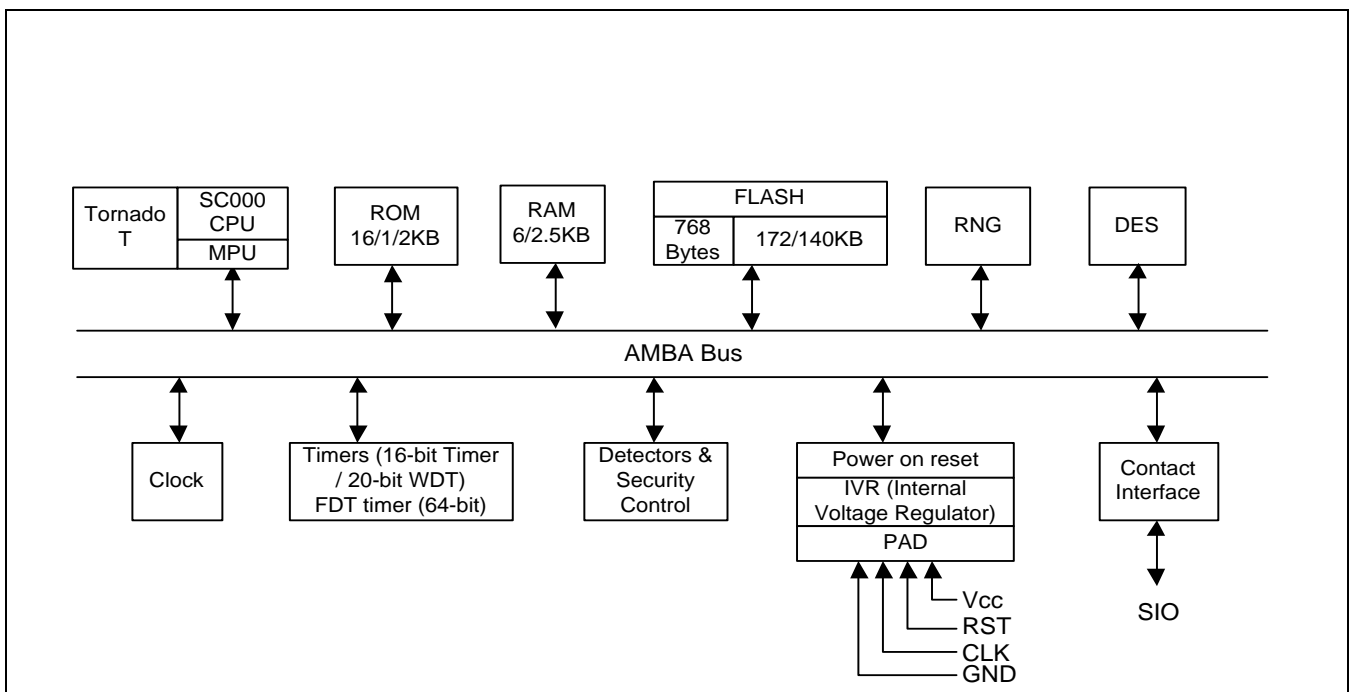
Figure 1 S3K170A/S3K140A Block Diagram
