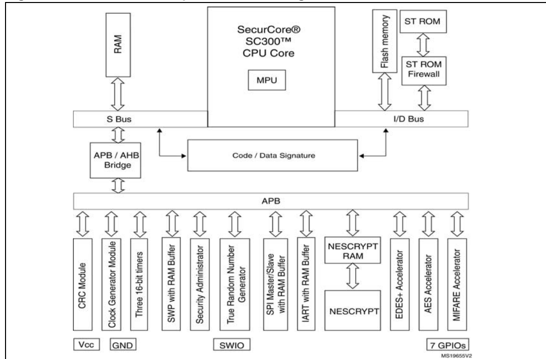
Figure 1. ST33G1M2 D01 platform block diagram
