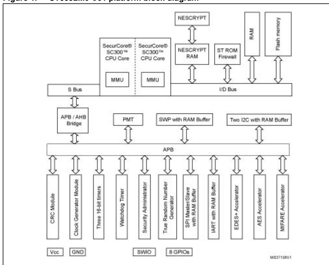
Figure 1. ST33J2M0 C01 platform block diagram
