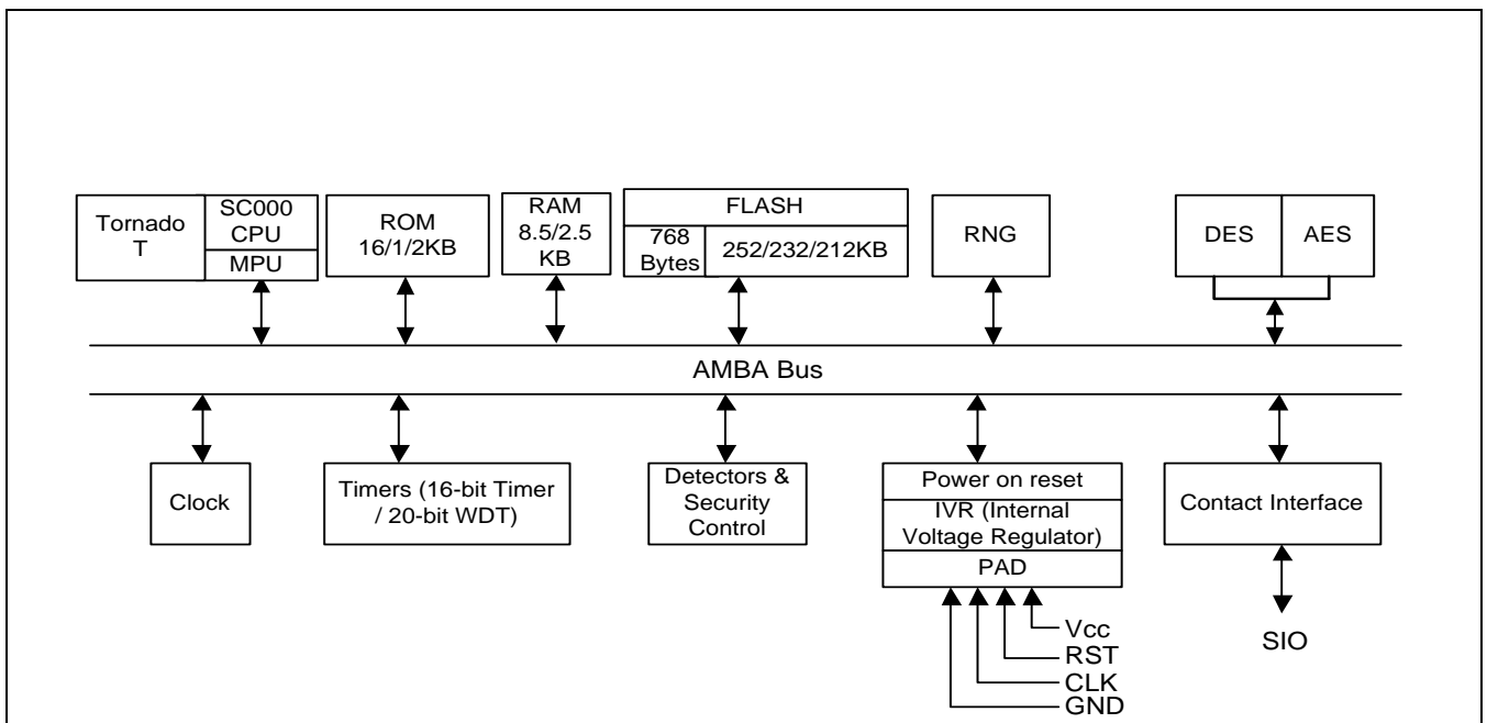
Figure 1 S3K250A/S3K232A/S3K212A Block Diagram
