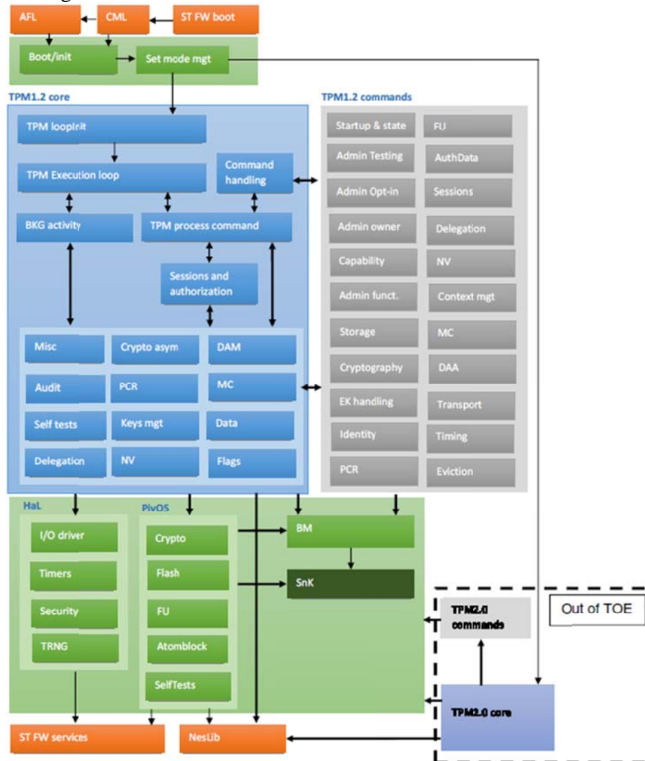
Figure 2 – Architecture logicielle
