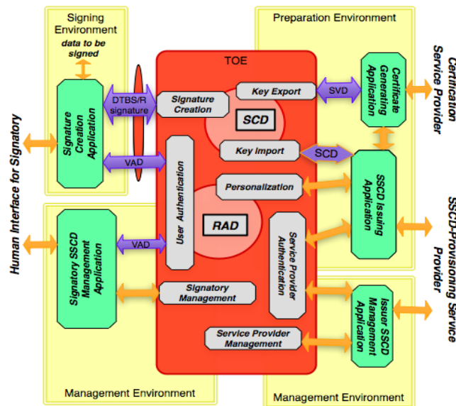
Figure 6: TOE and Operational environments with Key Import and trusted channel to SCA
