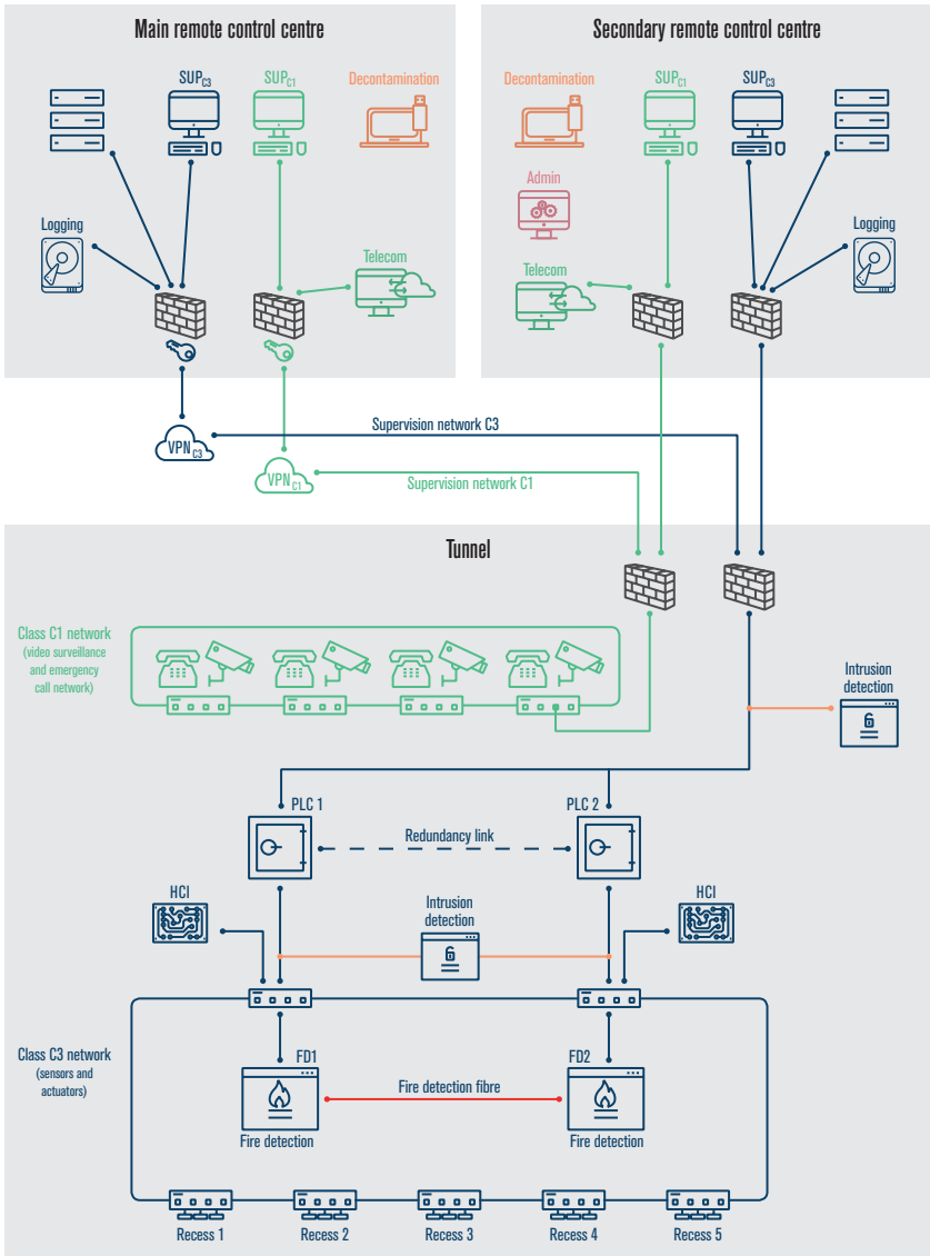
Figure 4 – Technical infrastructure view of the information system
