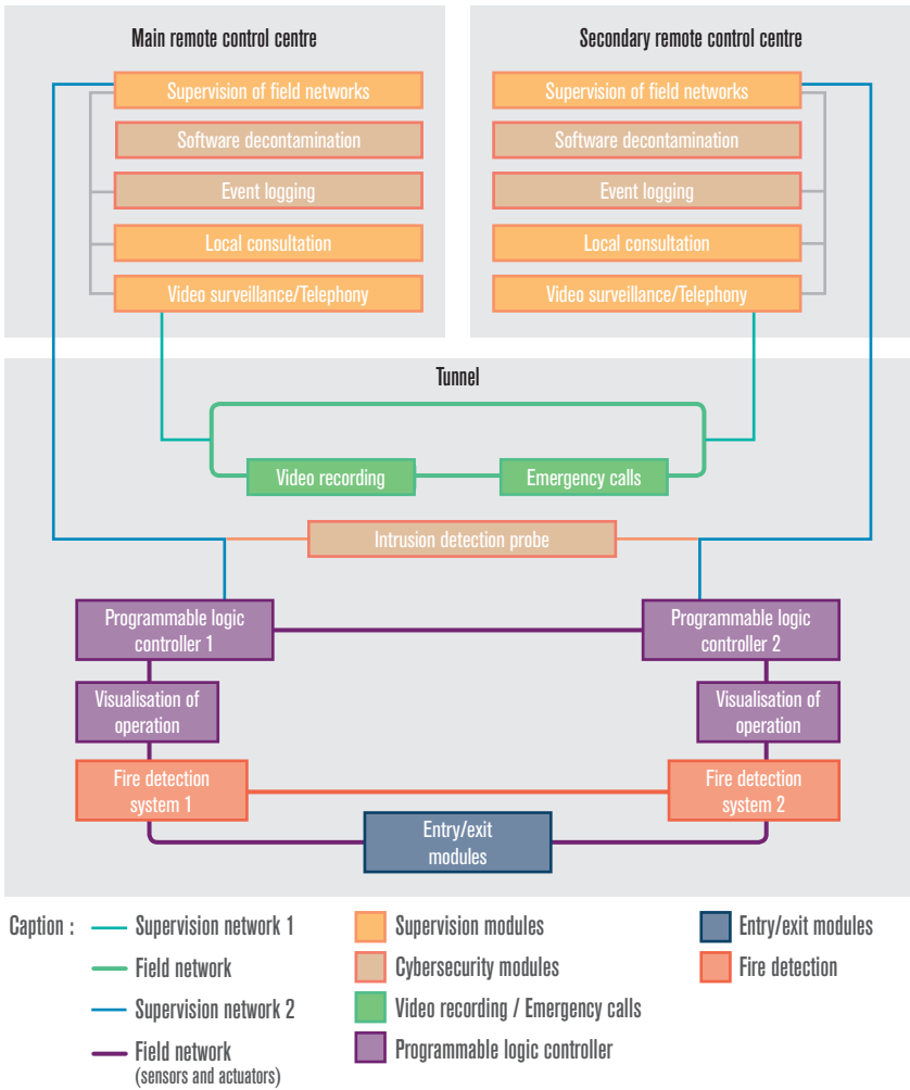
Figure 3 – Application view of the information system
