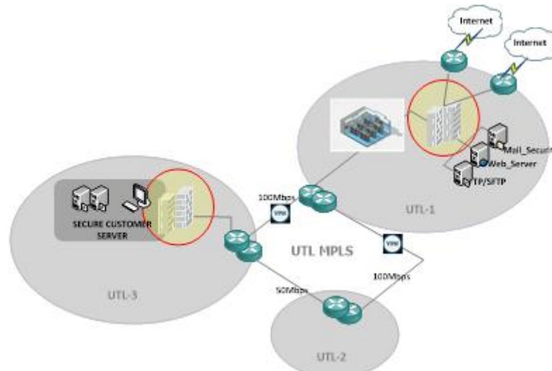
Figure 5 UTL Security Architecture Protections
