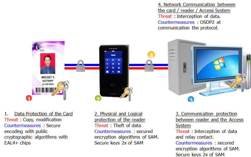
Figure 2 UTL Security for Badge & Reader
