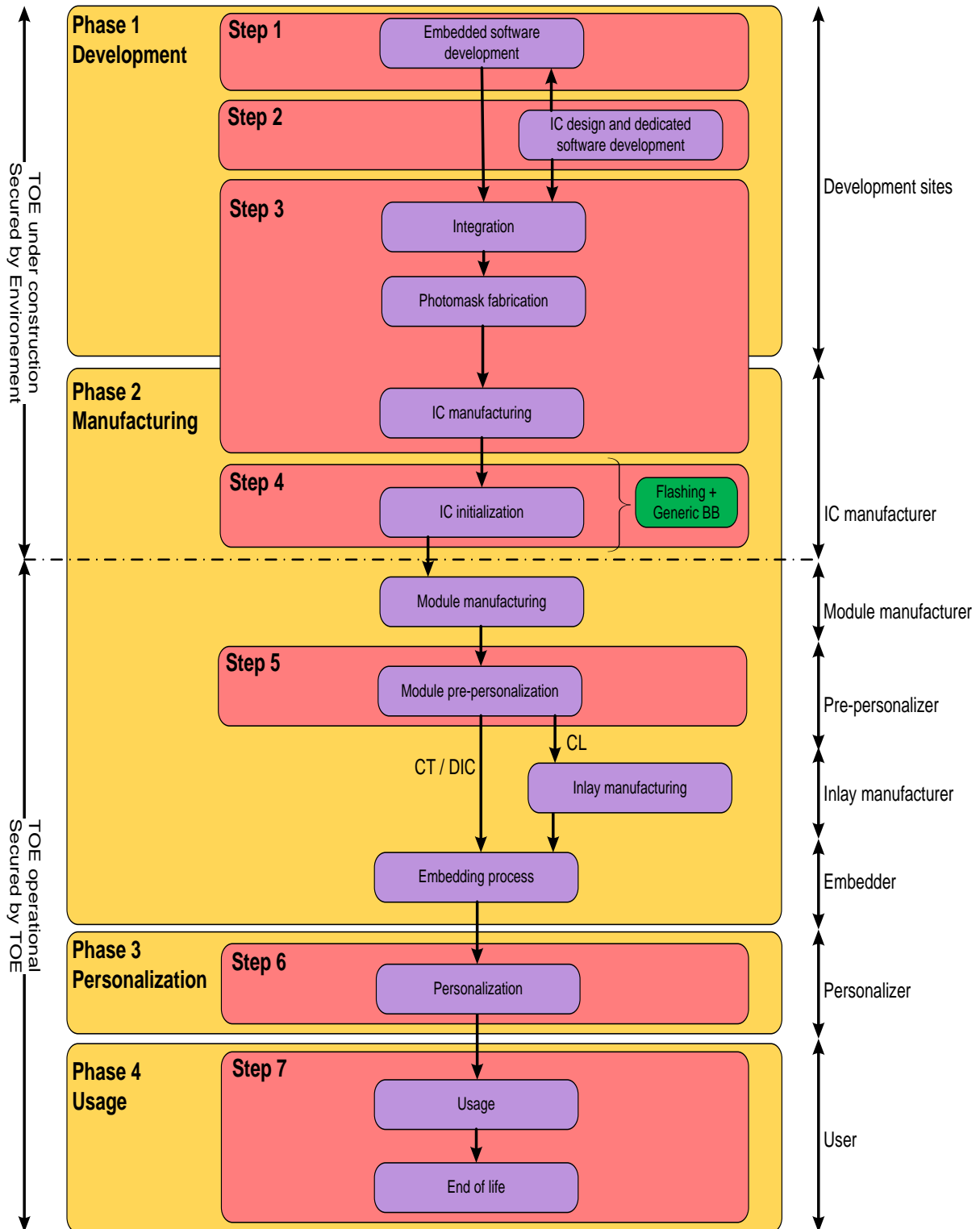
Figure 4 – Flashing and generic BlackBox loading at founder site on wafer; pre-personalization on module
