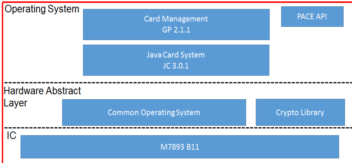
Figure 2 – Product architecture
