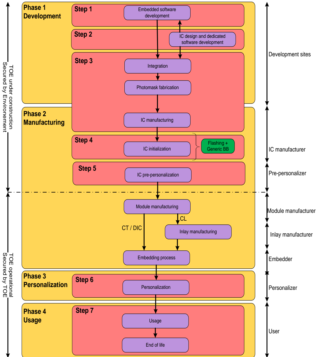
Figure 5 – Flashing and dedicated BlackBox loading at founder site on wafer; pre-personalization on IC
