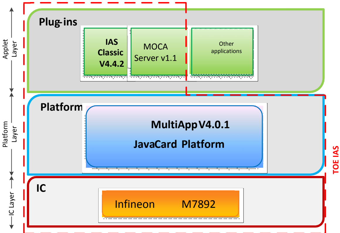
Figure 1: TOE Boundaries
