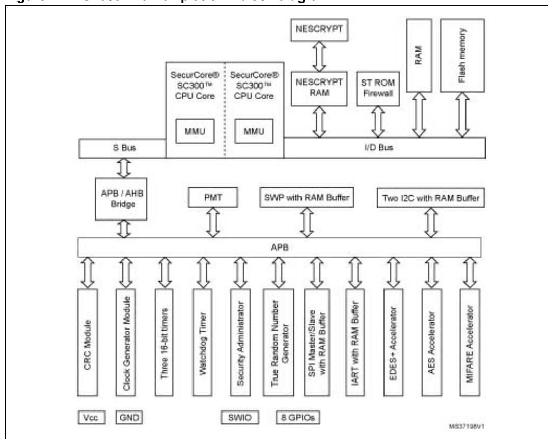
Figure 1. ST33J2M0 A02 platform block diagram
