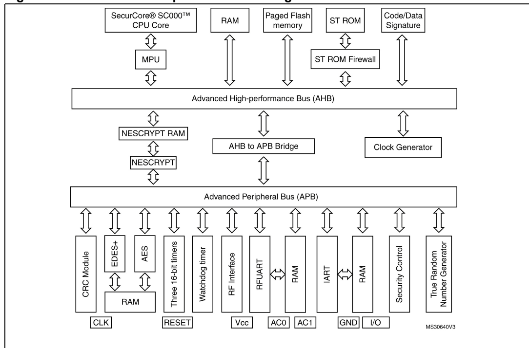
Figure 1. ST31G480 A05 platform block diagram
