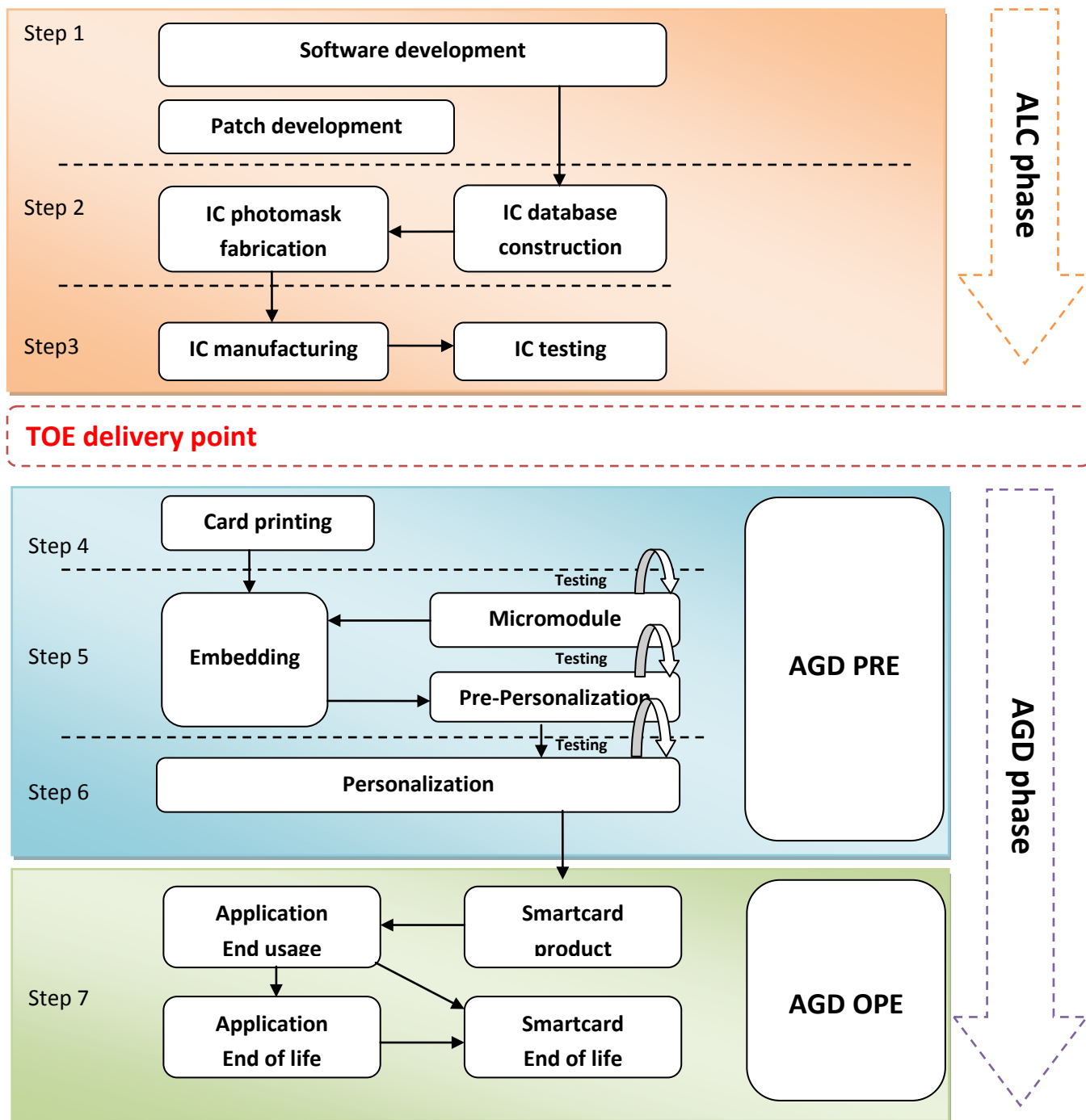
Figure 3 - TOE Lifecycle
