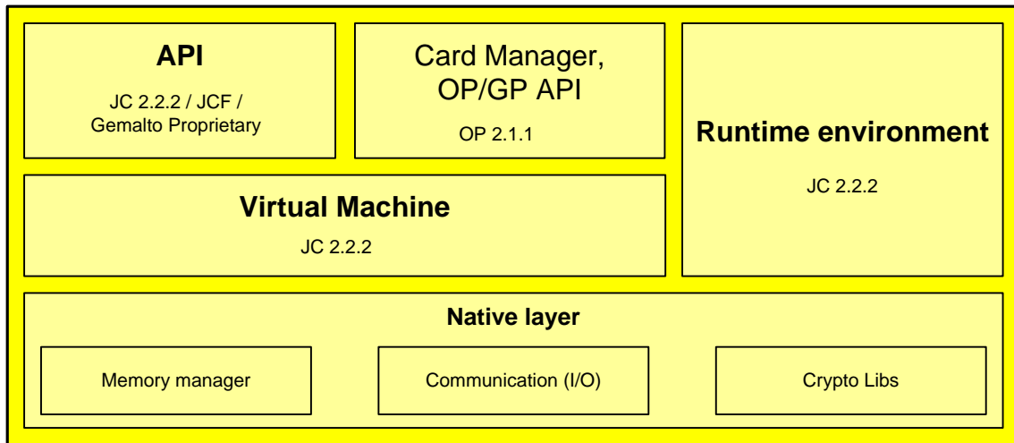
Figure 3: MAV31S Open Platform JCS architecture
