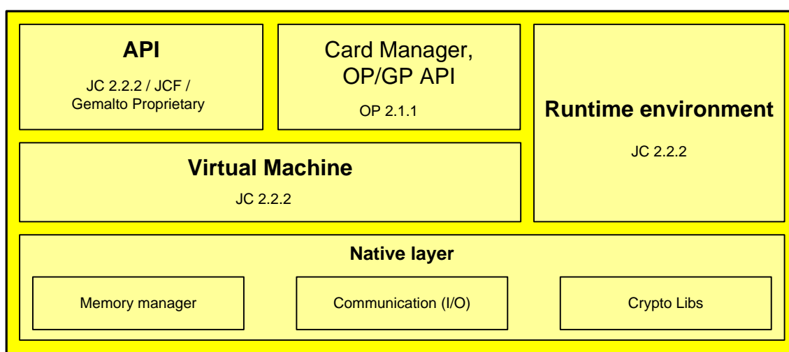
Figure 3: MultiApp ID V3.1 javacard platform architecture
